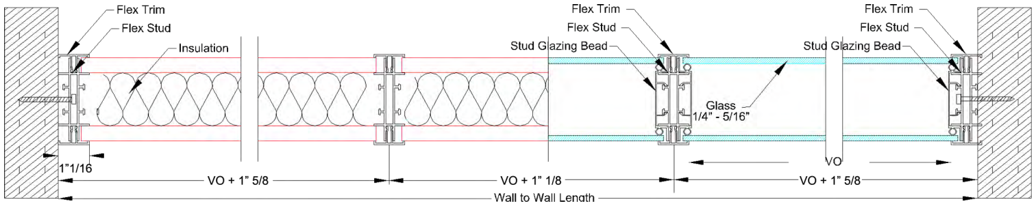
Detail B-B
