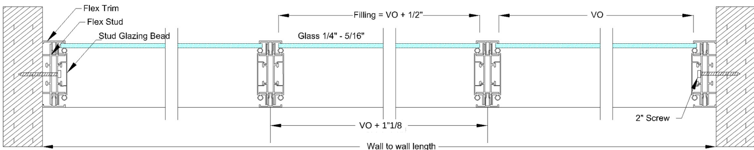
Detail B-B
