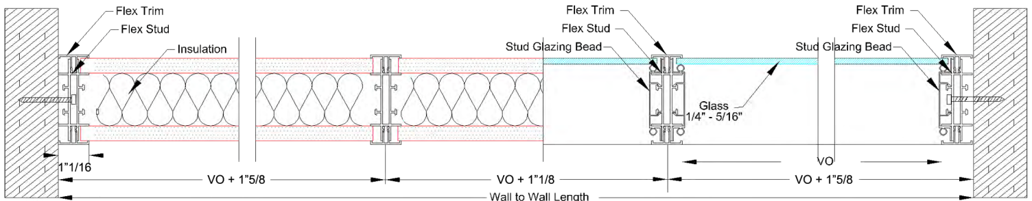
Detail B-B
