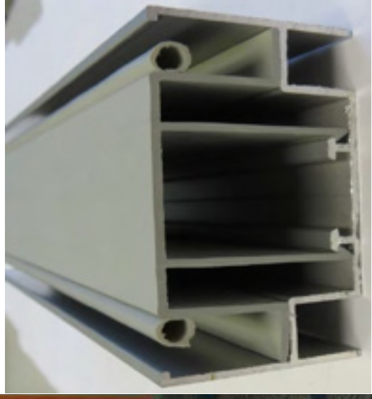
Track bead snapping into Floor or Ceiling Track
